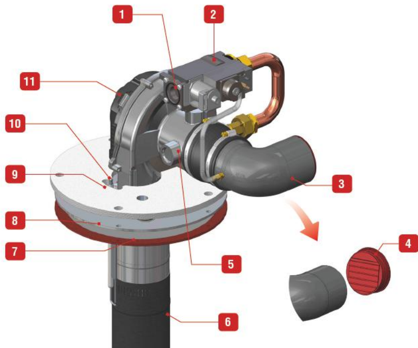
HeatMaster® 120 TC
