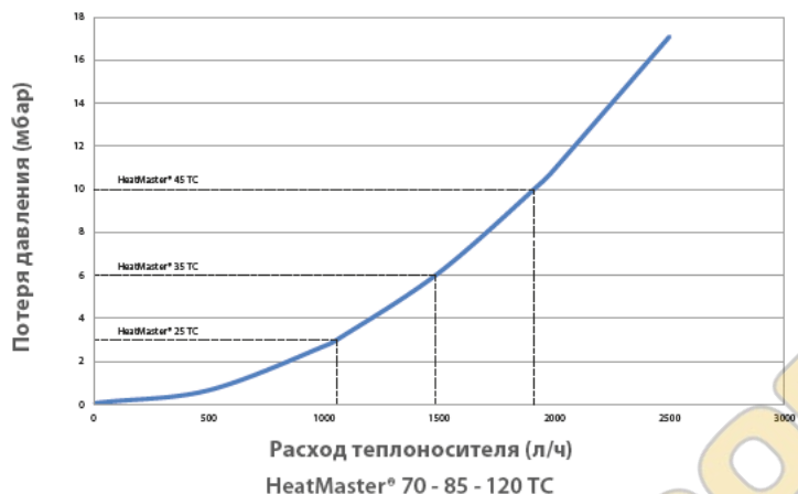
HeatMaster® 70 - 85 - 120 TC
