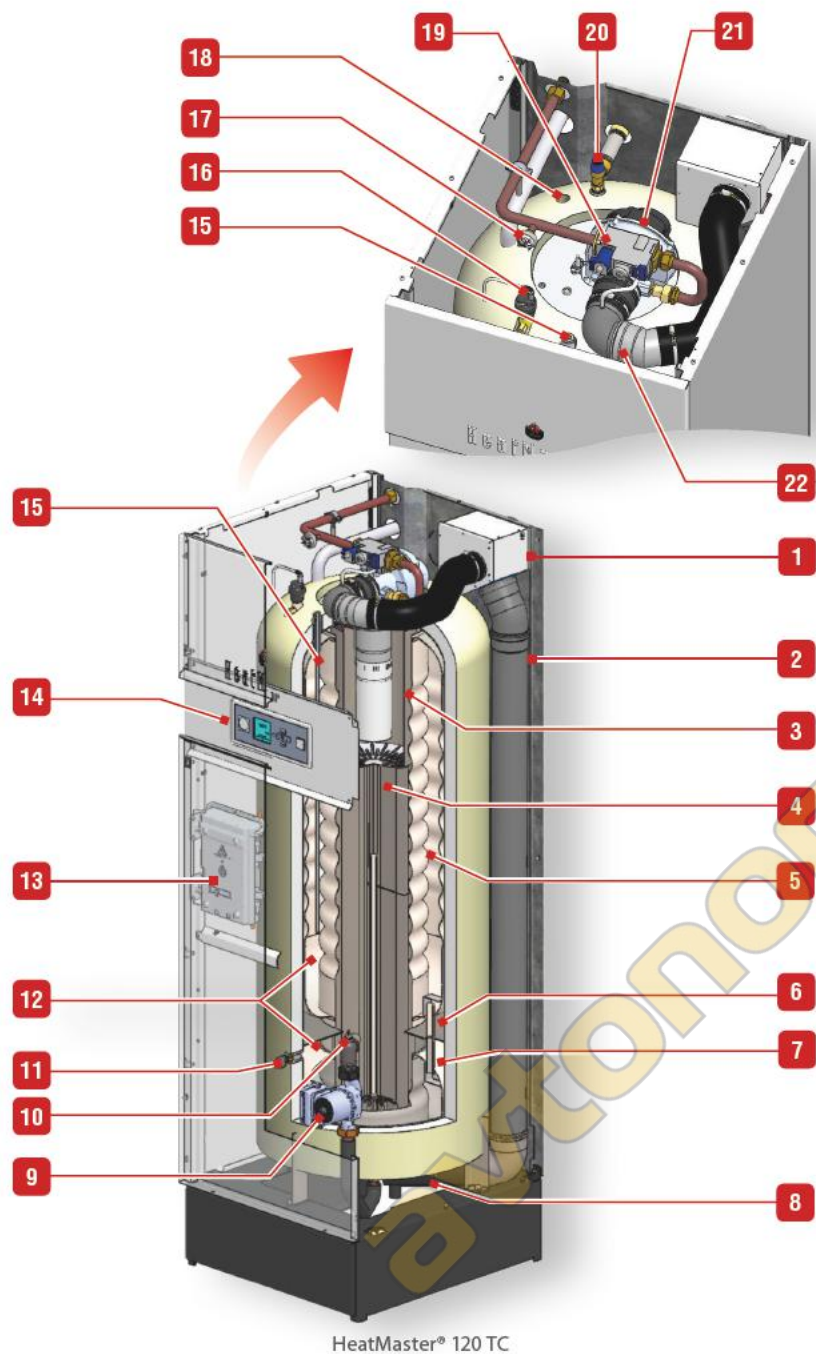
HeatMaster® 120 TC
