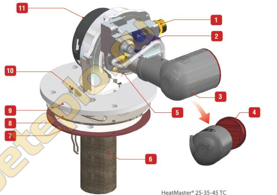
HeatMaster® 25-35-45 TC
